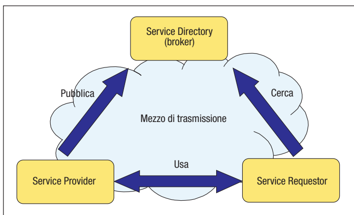
FIGURA 1 Service Oriented Architecture
